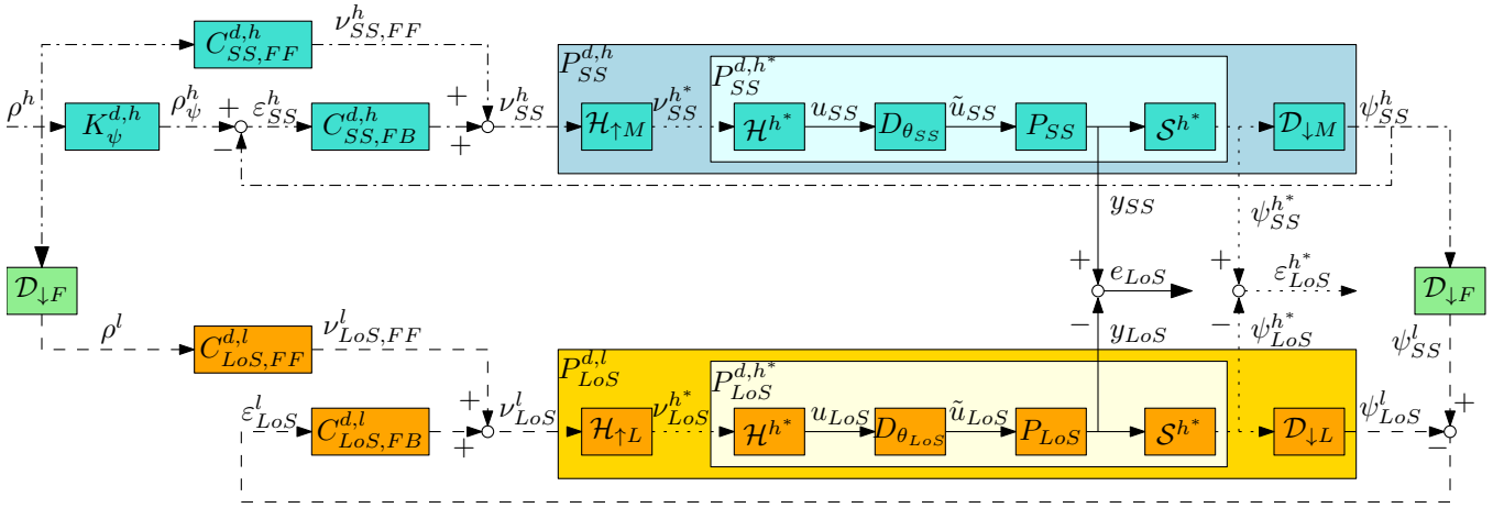
Fig. 4. The multi-rate control configuration for a wafer stage system. The short stroke system P_{SS}^{d,h} runs at high sampling frequency f^h with input shaping K_\psi^{d,h} and feedforward control C_{SS,FF}^{d,h} . The long stroke system P_{LoS}^{d,l} runs at low sampling frequency f^l with feedforward control C_{LoS,FF}^{d,l} to be designed.
