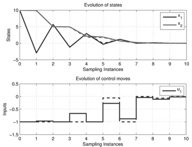
Fig. 6 Simulation of closed-loop ( \tilde{u} solid, u dashed)
