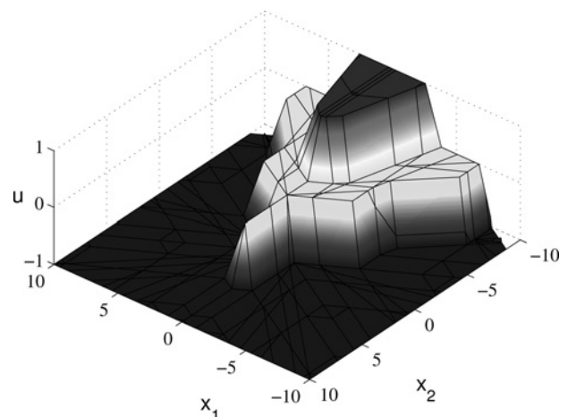
Fig. 4 Optimal control law u
