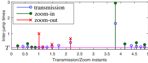
Fig. 3. Transmission/Zoom instants for the first 5 s.
