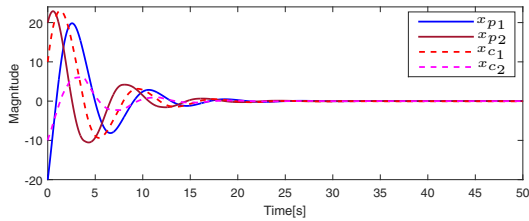
Fig. 2. State trajectory for the plant and the controller.
